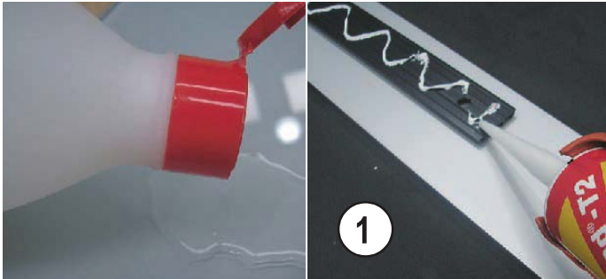
CLEAN BOTH SURFACES USING ALCOHOL. APPLY A UNIFORM THREAD OF CONSTRUCTION ADHESIVE.
