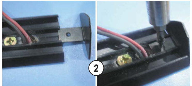
SCREW IN THE END CAPS INSERTING THEM IN THE CORRESPONDING GROOVES.
